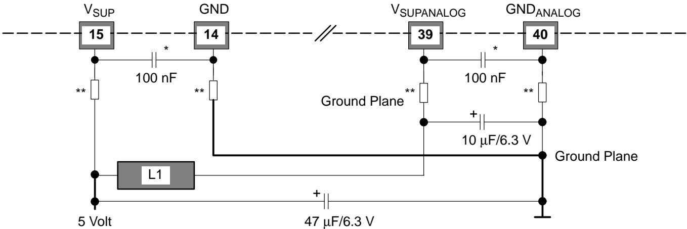
Fig. 6-2: Perfect grounding layout
