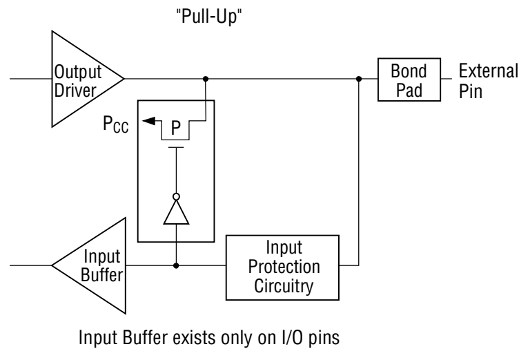
Figure 6b. Bus Hold Circuit Pin 26-32, 34
