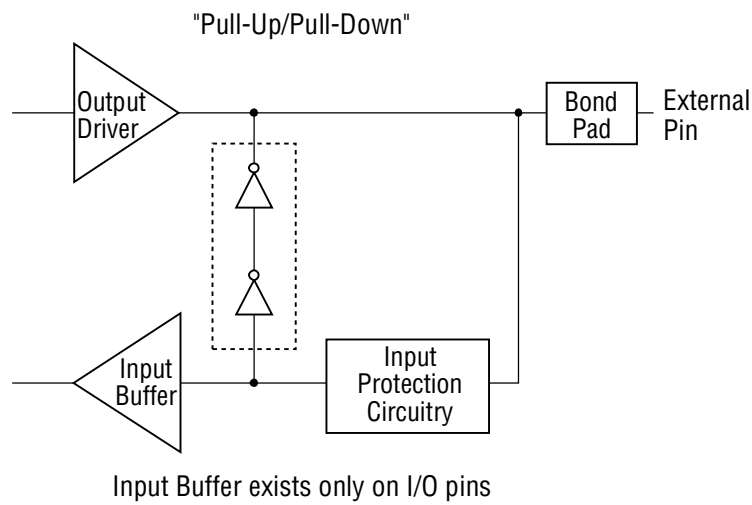
Figure 6a. Bus Hold Circuitry Pin 2-16, 35-39
