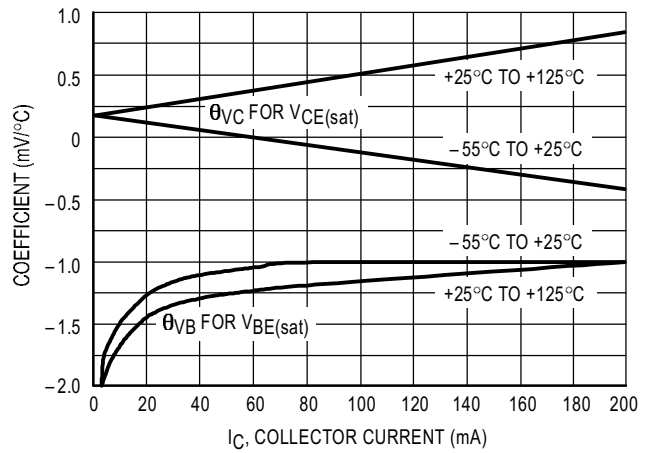
Figure 18. Temperature Coefficients
