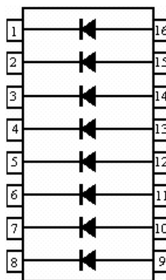
CIRCUIT CONFIGURATION
