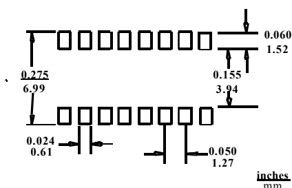
PAD LAYOUT
