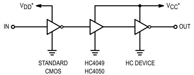
High-Voltage CMOS to HSCMOS
