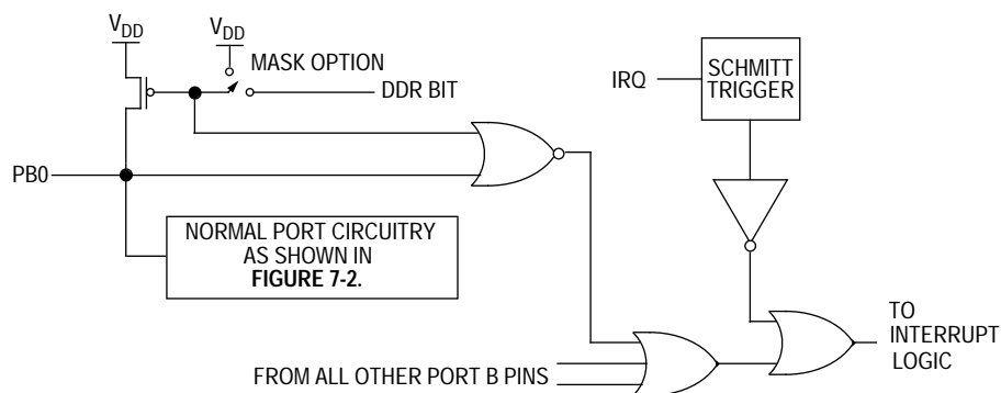
Figure 7-1. Port B Pullup Option
