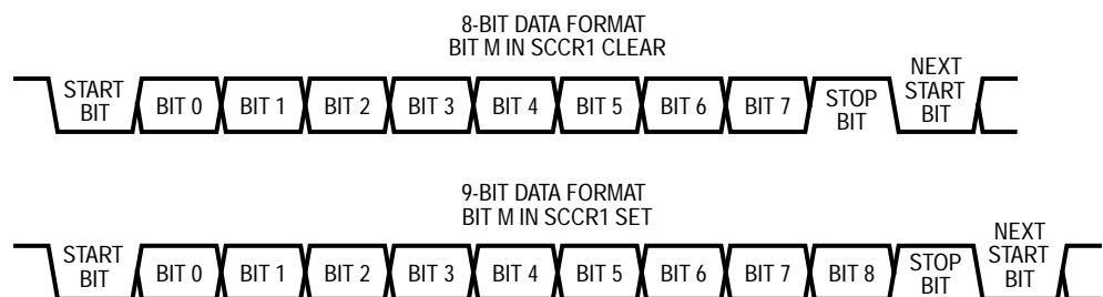
Figure 9-1. SCI Data Format
