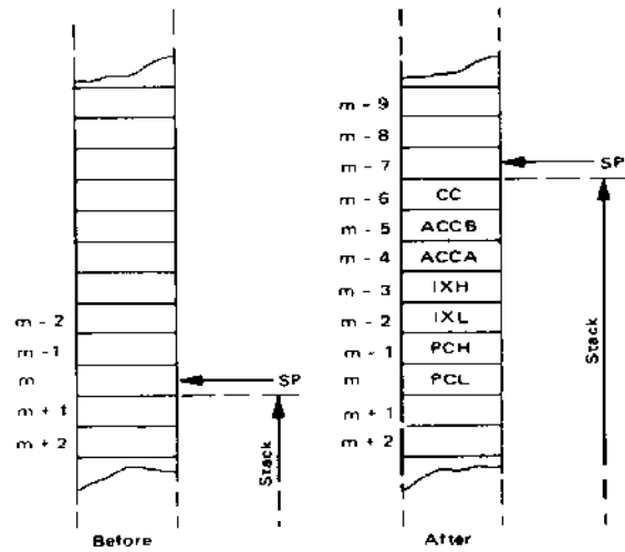
FIGURE B — SAVING THE STATUS OF THE MICROPROCESSOR IN THE STACK
