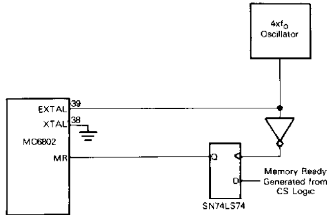
FIGURE 14 — MEMORY READY SYNCHRONIZATION
