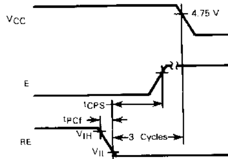
FIGURE 10 — POWER-DOWN SEQUENCE
