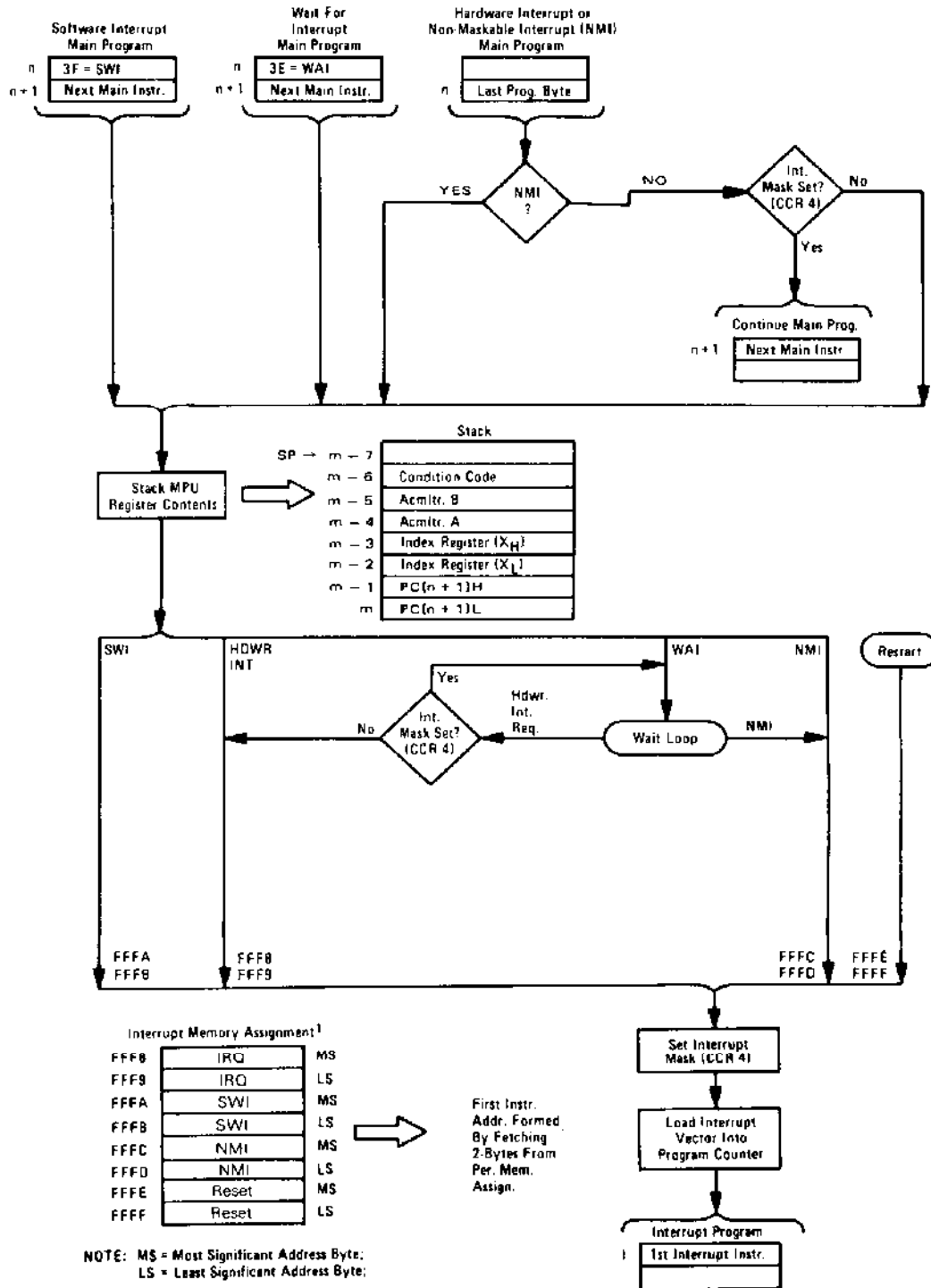
FIGURE 23 — PROGRAM FLOW FOR INTERRUPTS
