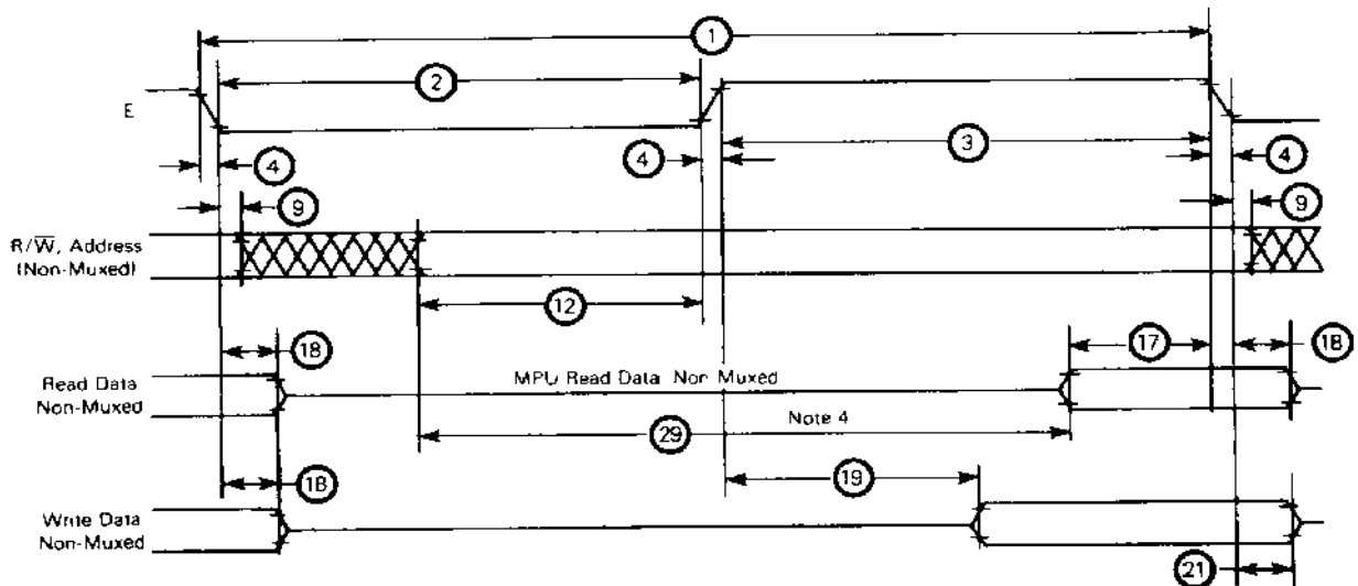
FIGURE 2 — BUS TIMING
