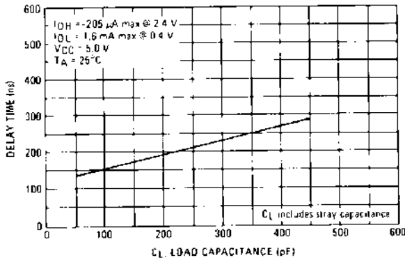
FIGURE 4 — TYPICAL DATA BUS OUTPUT DELAY versus CAPACITIVE LOADING
