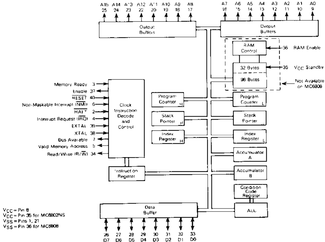
FIGURE 6 — EXPANDED BLOCK DIAGRAM
