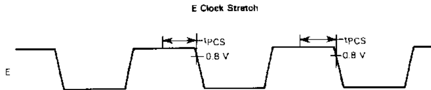
FIGURE 15 — MR NEGATIVE SETUP TIME REQUIREMENT
