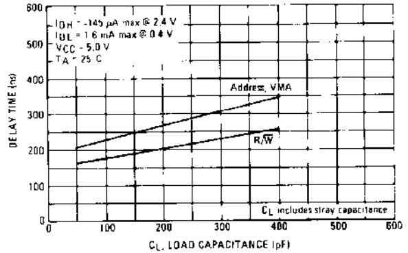
FIGURE 5 — TYPICAL READ/WRITE, VMA AND ADDRESS OUTPUT DELAY versus CAPACITIVE LOADING
