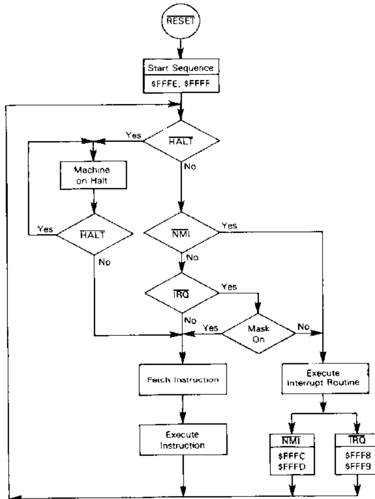
FIGURE 11 — MPU FLOWCHART
