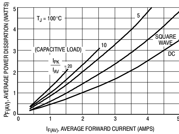
Figure 3. Power Dissipation
