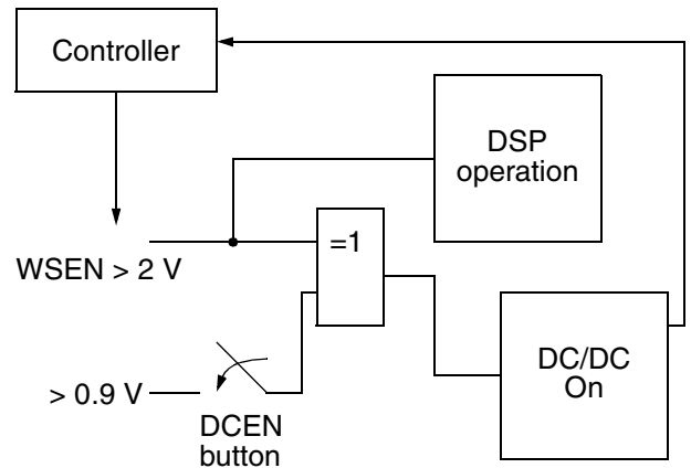
Fig. 2-3: DC/DC operation
