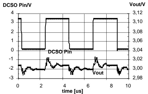
Switching Waveforms
