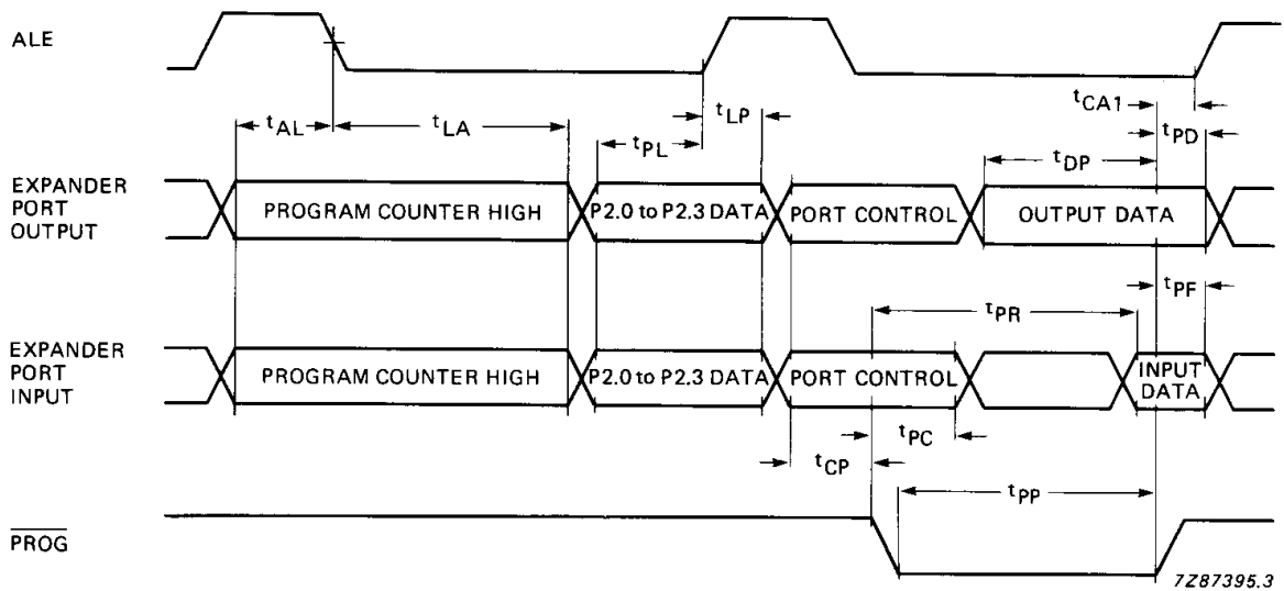
Fig. 17 Port 2 timing.
