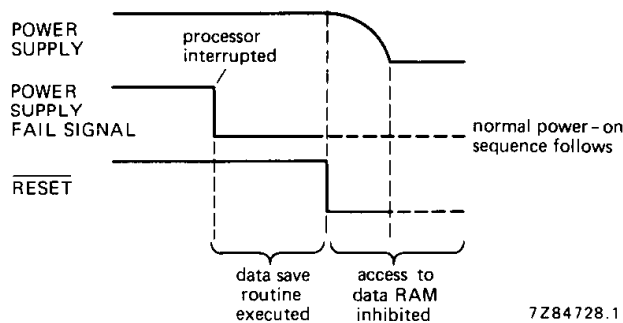
Fig. 10 Power down sequence.
