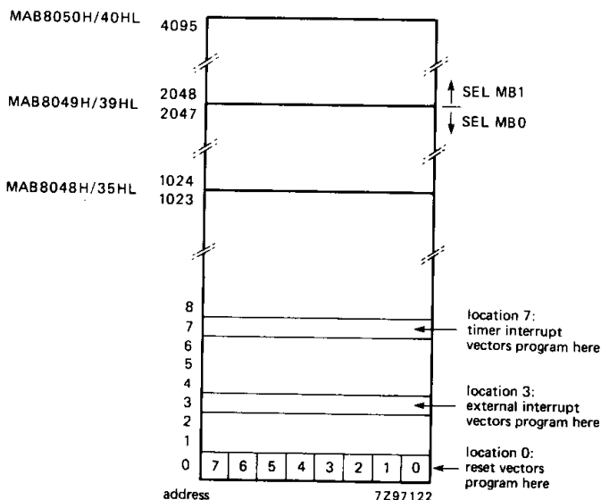
Fig. 3 Program memory map.
