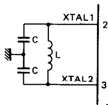
Fig. 7 LC oscillator. Each capacitor should be \approx 20 pF including stray capacitance C_{pp} \approx 5 to 10 pF (pin-to-pin capacitance).
