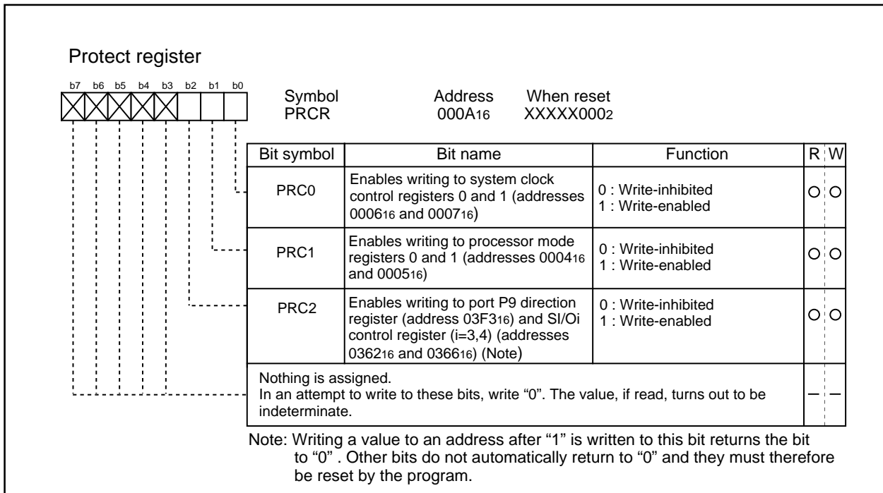
Figure 1.10.6. Protect register
