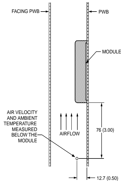
Figure 30. Experimental Test Setup
