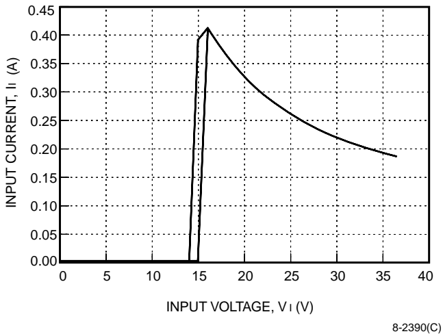
Figure 1. LC005x Input Current vs. Input Voltage at I_o = I_{o, max} and T_c = 25\text{ }^\circ\text{C}
