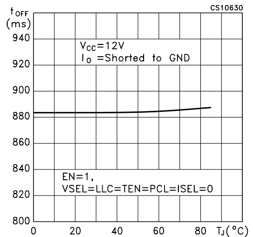
Figure 13 : Dynamic Overload Protection OFF Time vs Temperature
