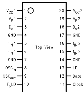
LMX2336L (Top View)
