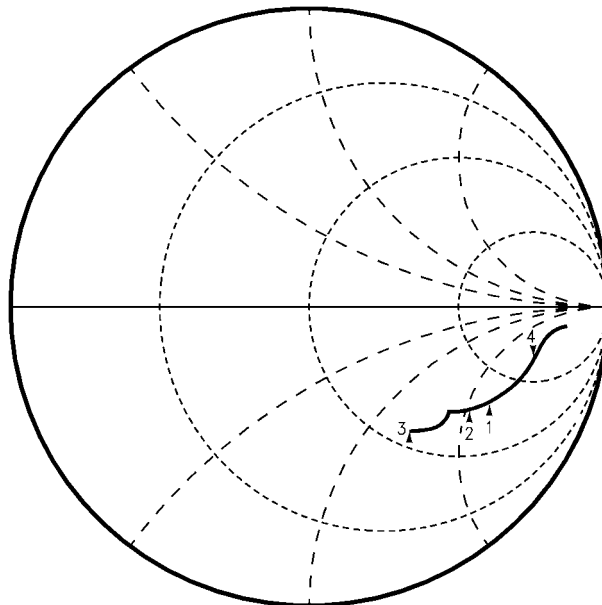
LMX2335L Input Impedance (for TSSOP package)
