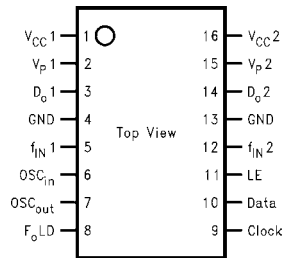
LMX2335L (Top View)
