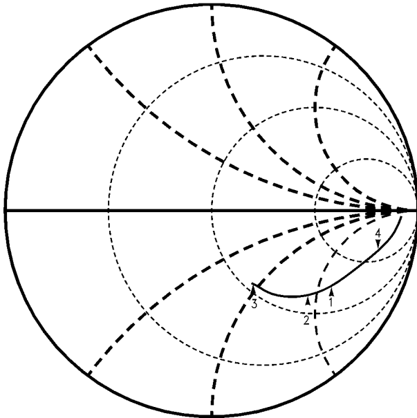
LMX2335L Input Impedance (for SO package)
