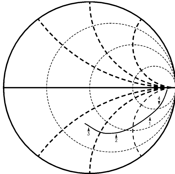
LMX2336L Input Impedance (for TSSOP package)
