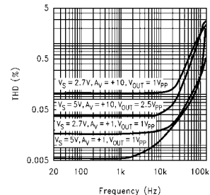
Frequency (Hz) DS100060-59
