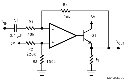
FIGURE 22. Power Amplifier
