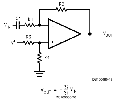
FIGURE 10. Single-Supply Inverting Amplifier
