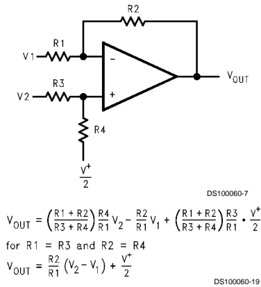
FIGURE 7. Difference Amplifier
