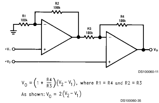
FIGURE 9. Two-Op-amp Instrumentation Amplifier
