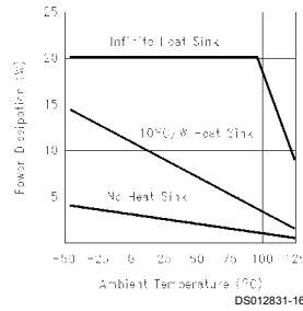
Maximum Power Dissipation (TO-220 Package)
