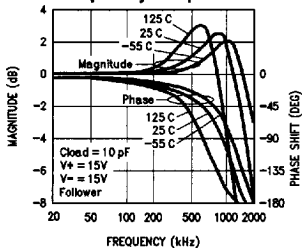
Follower Small-Signal Frequency Response
