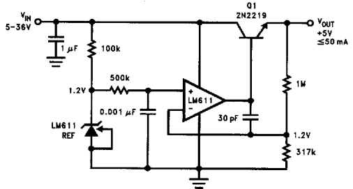
TL/H/9221-30 FIGURE 13. Simple Low Quiescent Drain Voltage Regulator. Total Supply Current is approximately 320 \mu A when V_{IN} = 5V , and output has no load.
