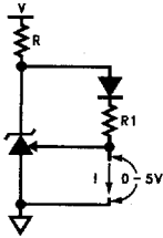
TL/H/9221-23 FIGURE 10. Proportional-to-Absolute-Temperature Current Source
