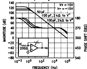
Small-Signal Voltage Gain vs Frequency and Load
