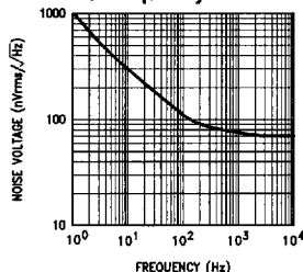
Op Amp Voltage Noise vs Frequency
