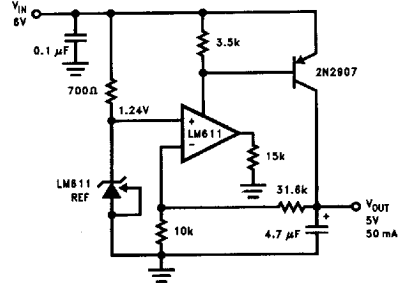
FIGURE 15. Low Drop-Out Voltage Regulator Circuit. Drop out voltage is typically 0.2V.
