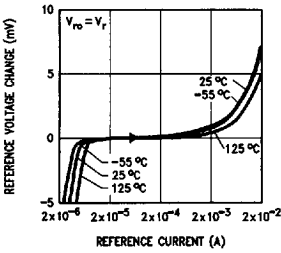
Reference Voltage vs Reference Current
