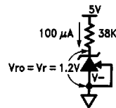
FIGURE 3. 1.2V Reference
