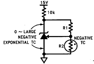
FIGURE 6. Output Voltage has Negative Temperature Coefficient (TC) if R2 has Negative TC
