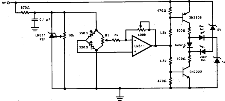
FIGURE 16. Nulling Bridge Detection System. Adjust sensitivity via 400 k Ω pot. Null offset with R1, and bridge drive with the 10k pot.
