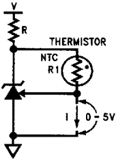
TL/H/9221-24 FIGURE 11. Negative -TC Current Source
