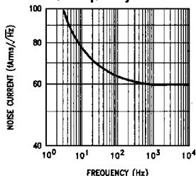
Op Amp Current Noise vs Frequency
