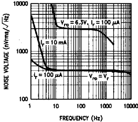
Reference Noise Voltage vs Frequency
