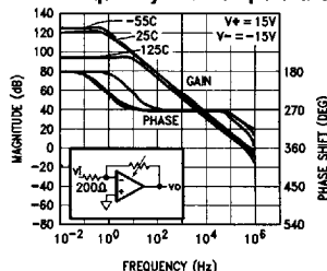
Small-Signal Voltage Gain vs Frequency and Temperature
