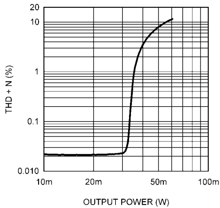
THD+N vs Output Power/Channel V_{DD} = 3V , R_L = 32\Omega , A_{V-SE} = 1V/V f = 1kHz , C_{OUT} = 220\mu F , 80kHz BW
