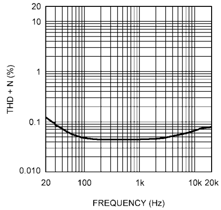
THD+N vs Frequency V_{DD} = 5V , R_{LDOCK} = 10k\Omega , Dock Pins V_{IN} = 1Vp-p , C_O = 1\mu F , 80kHz BW
