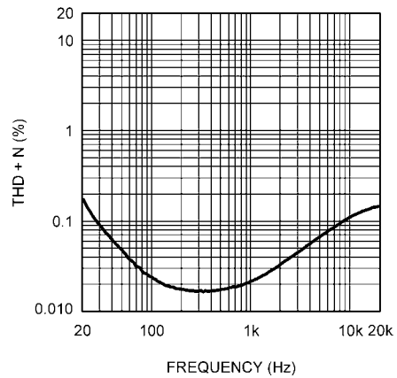
THD+N vs Frequency V_{DD} = 3V , R_L = 32\Omega , A_{V-SE} = 1V/V P_{OUT} = 20mW/Channel , 80kHz BW
