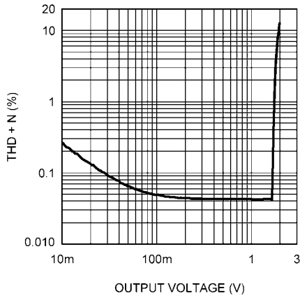
THD+N vs Output Voltage V_{DD} = 5V , R_{LDOCK} = 10k\Omega , Dock Pins f = 1kHz , C_O = 1\mu F , 80kHz BW
