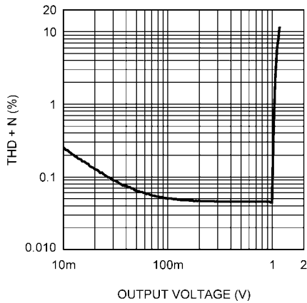
THD+N vs Output Voltage V_{DD} = 3V , R_{LDOCK} = 10k\Omega , Dock Pins f = 1kHz , C_O = 1\mu F , 80kHz BW
