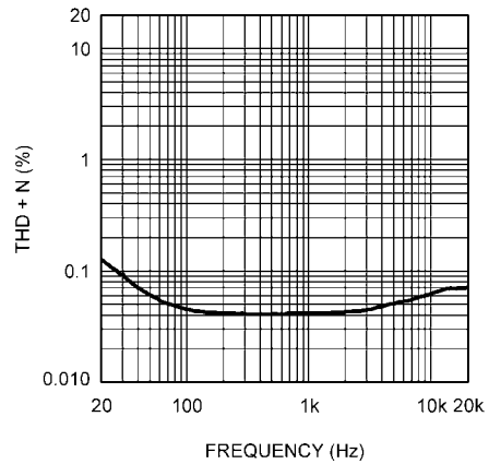
THD+N vs Frequency V_{DD} = 3V , R_{LDOCK} = 10k\Omega , Dock Pins V_{IN} = 1Vp-p , C_O = 1\mu F , 80kHz BW
