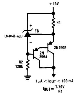
FIGURE 10. Current Source
