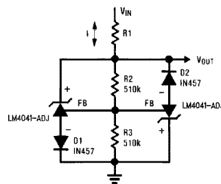
FIGURE 7. Bidirectional Clamp \pm 2.4V
