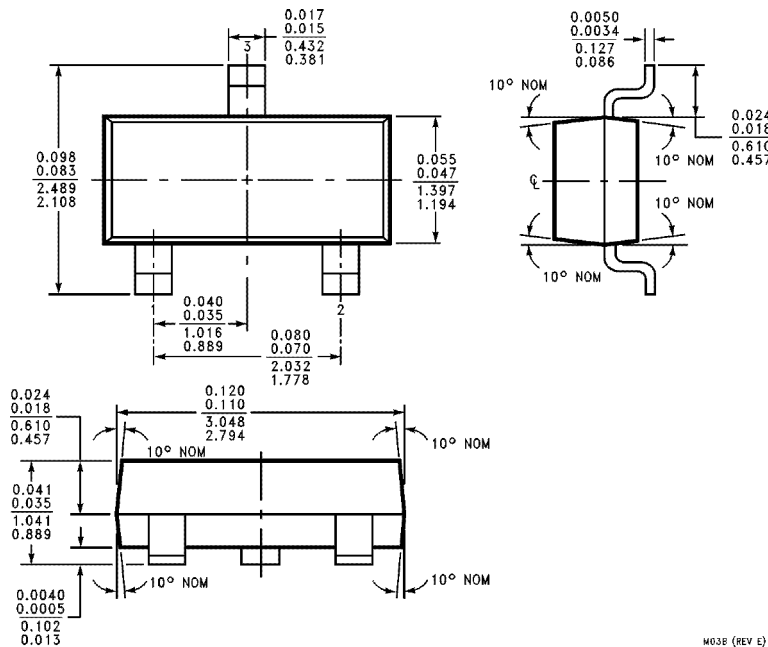
Plastic Surface Mount Package (M3) NS Package Number M03B (JEDEC Registration TO-236AB)
