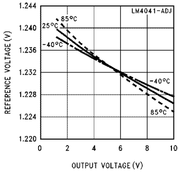
Reference Voltage vs Output Voltage and Temperature
