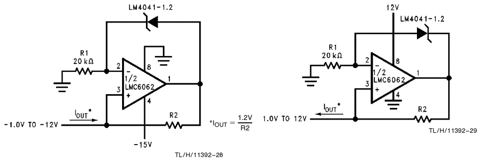
FIGURE 13. Precision 1 \mu A to 1 mA Current Sources
