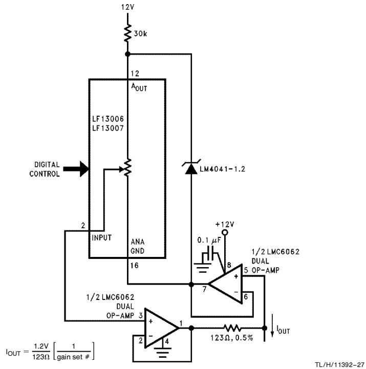
FIGURE 12. Programmable Current Source
