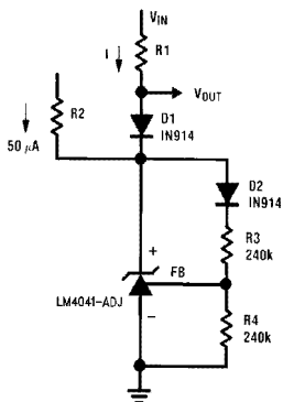
FIGURE 6. Fast Positive Clamp 2.4V + \Delta V_{D1}
