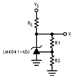
FIGURE 2. Adjustable Shunt Regulator
