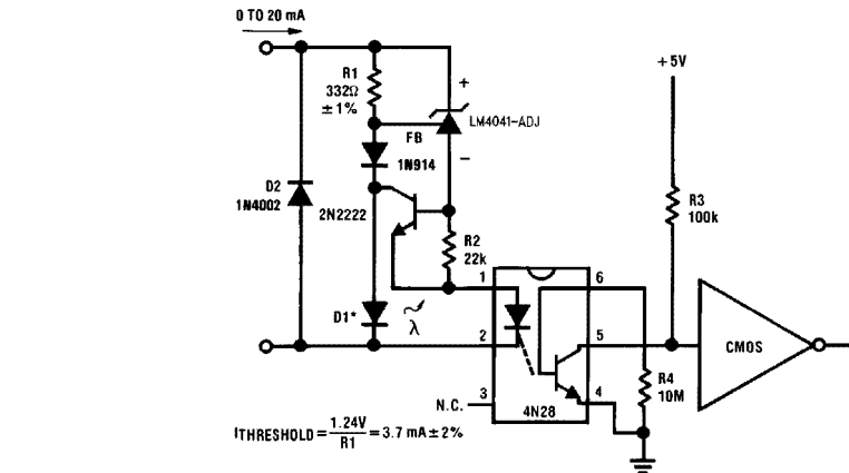
FIGURE 11. Precision Floating Current Detector
