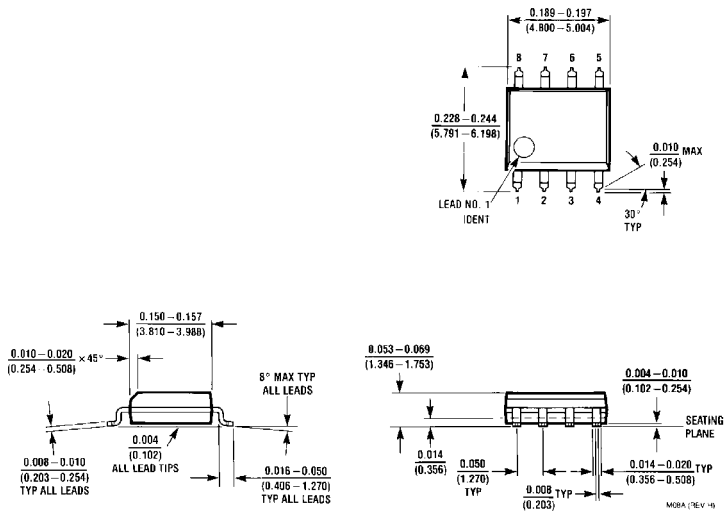
Dual-In-Line Package (M) Order Number LM211M or LM311M NS Package Number M08A
