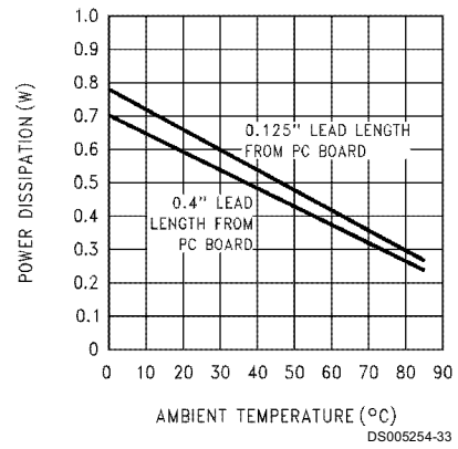
Maximum Power Dissipation (TO-92)
