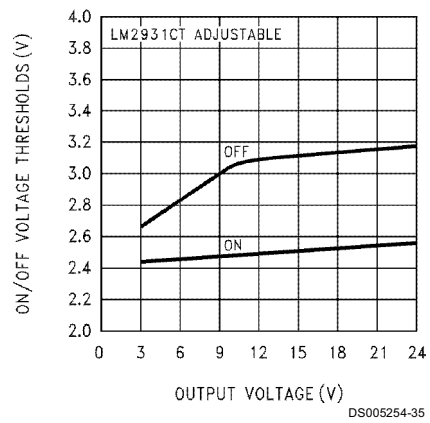
On/Off Threshold
