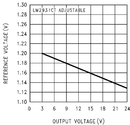
Reference Voltage
