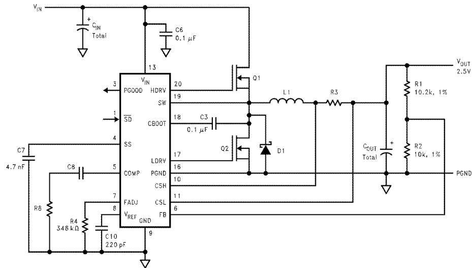
FIGURE 2. The Typical 2.5V Application Circuit
