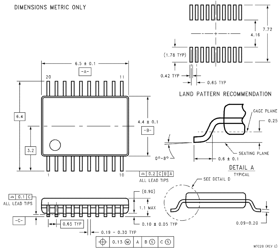
20-Lead TSSOP (MTC) Order Number LM2631MTC-ADJ NS Package Number MTC20
