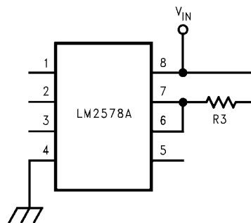
FIGURE 3. Current Limit, V_{in} Referred
