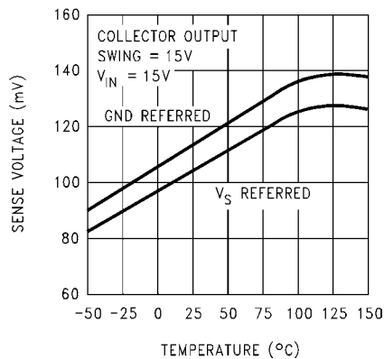
Current Limit Sense Voltage Drift with Temperature
