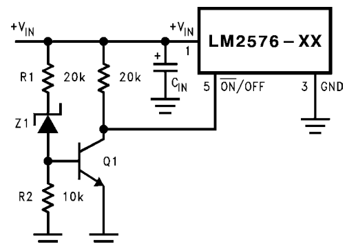
FIGURE 12. Undervoltage Lockout for Buck Circuit
