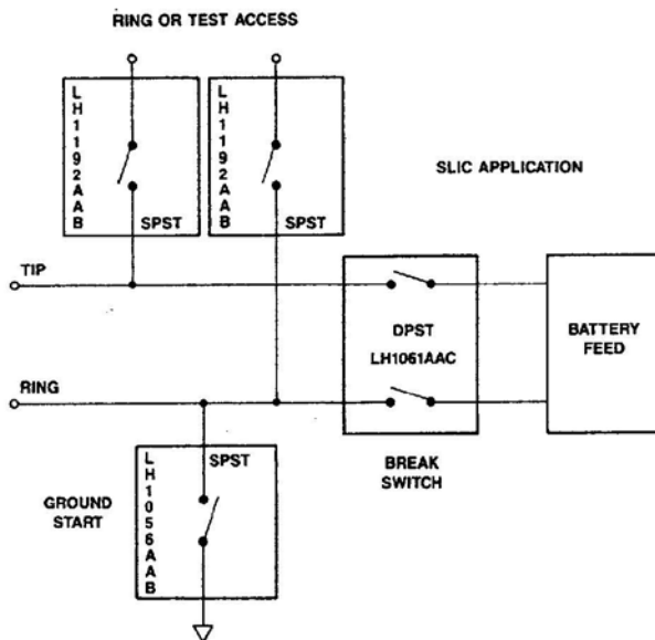
Figure 7. SLIC Application
