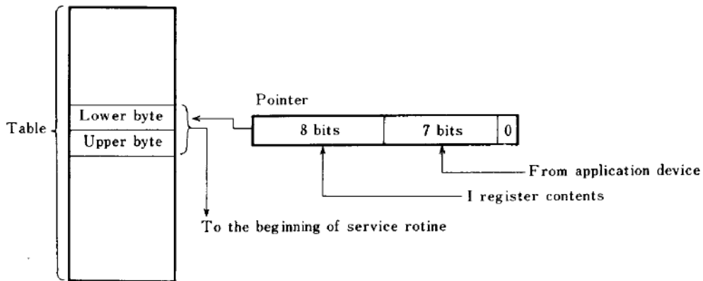
Fig. 1 Mode 2 interrupt diagram
