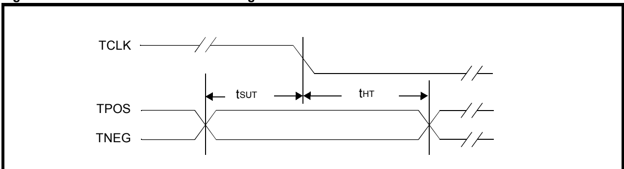
Figure 19: LXT332 Transmit Clock Timing
