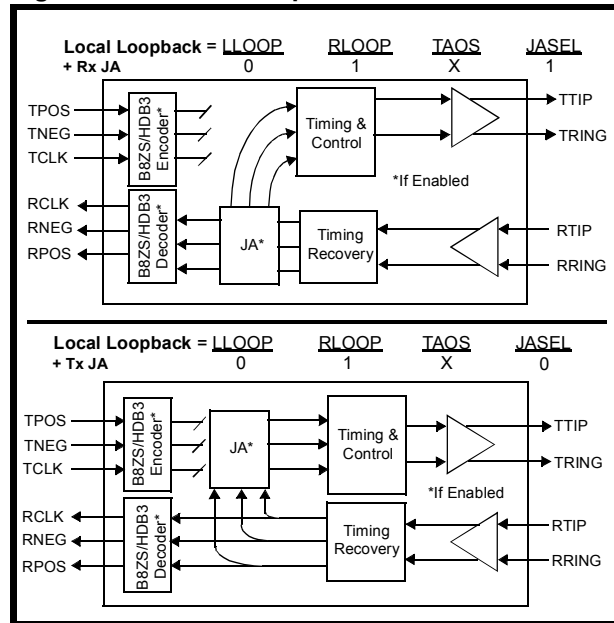
Figure 11: Dual Loopback
