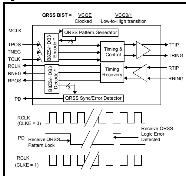
Figure 12: QRSS BIST Mode
