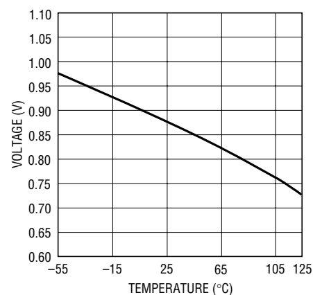
Shutdown Threshold
