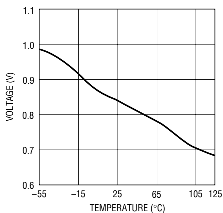
Start-Up Voltage
