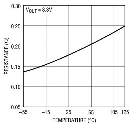
PMOS R_{DS(ON)}
