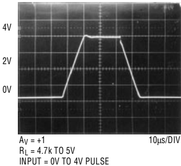
Large Signal Transient Response, V_S = 5\text{V}, 0\text{V}
