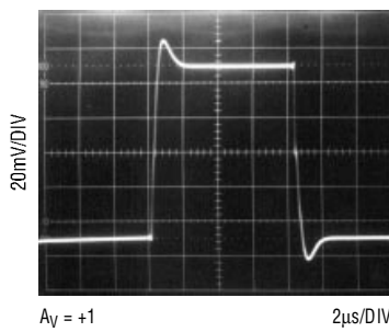
Small Signal Transient Response, V_S = \pm 15\text{V}
