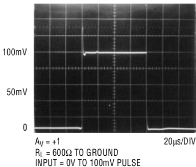
Small Signal Transient Response, V_S = 5\text{V}, 0\text{V}
