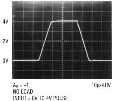
Large Signal Transient Response, V_S = 5\text{V}, 0\text{V}
