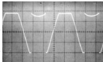
LM324, LM358, OP-20 EXHIBIT OUTPUT PHASE REVERSAL
