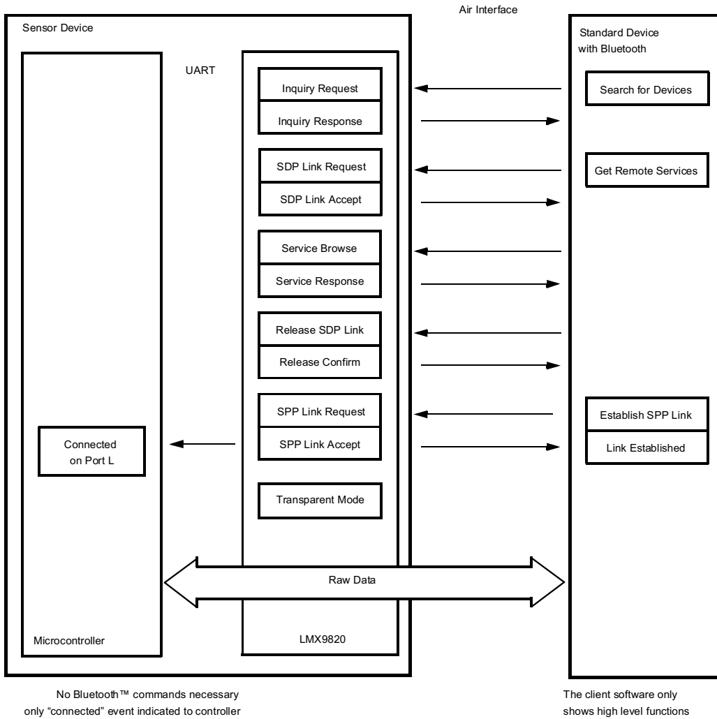
Figure 18. Point-to-Point Connection
