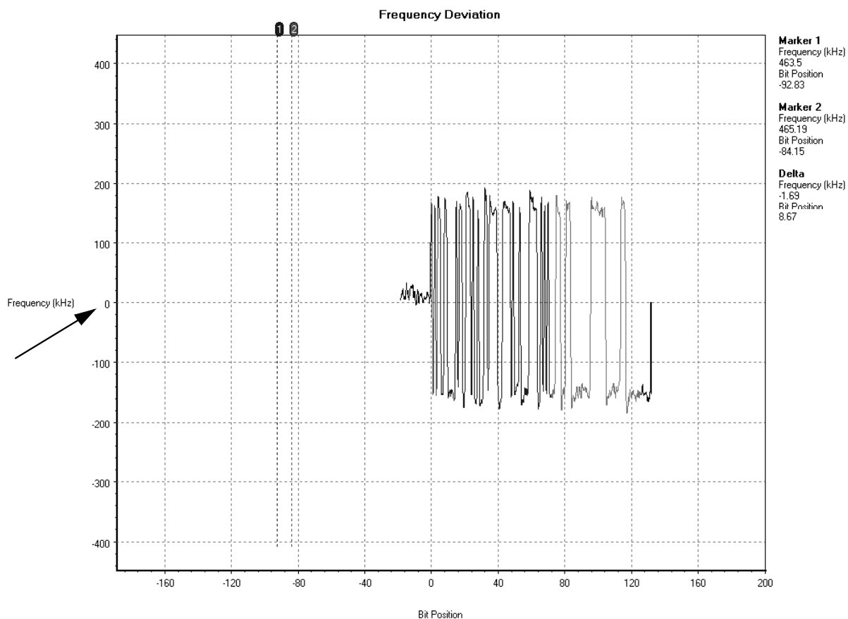
Figure 13. Frequency Offset with 9 pF//10 pF Capacitors
