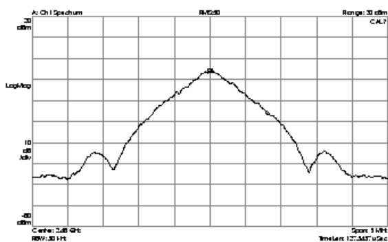
Figure 4. Transmit Spectrum
