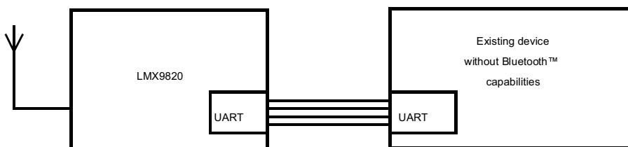
Figure 17. Bluetooth Functionality
