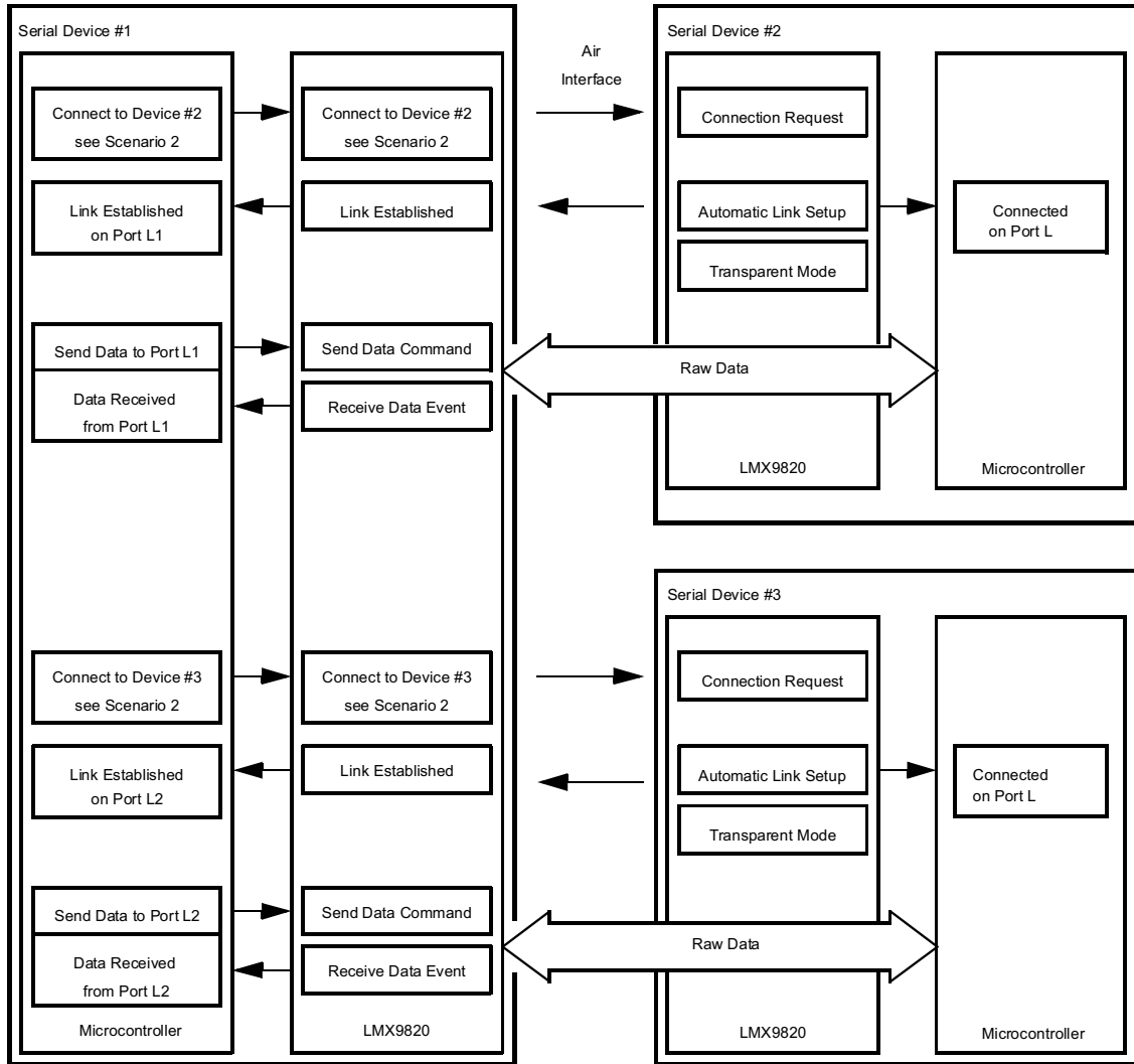
Figure 20. Point-to-Multipoint Connection
