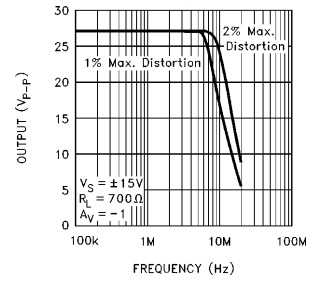
Undistorted Output Swing vs Frequency
