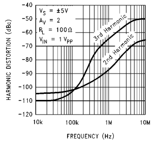
Harmonic Distortion vs Frequency
