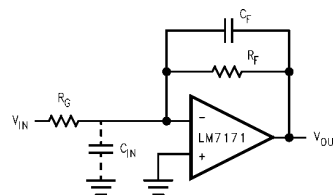
FIGURE 1. Compensating for Input Capacitance
