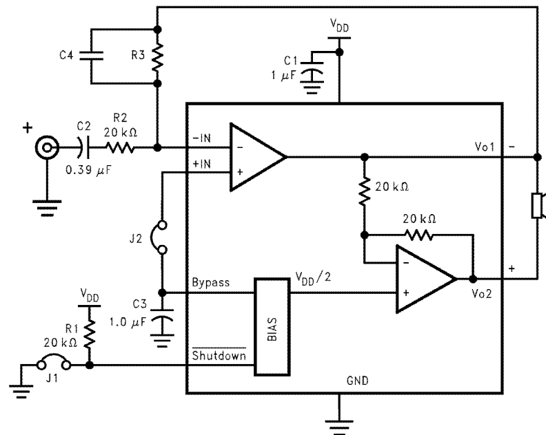
FIGURE 2. HIGHER GAIN AUDIO AMPLIFIER
