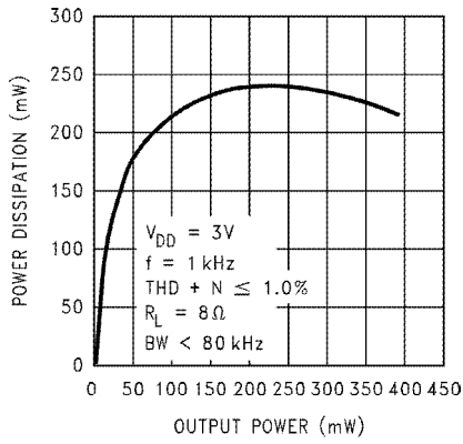
Power Dissipation vs Output Power V_{DD} = 3V
