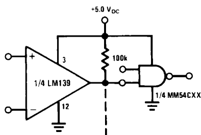
Driving CMOS
