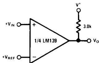
Basic Comparator
