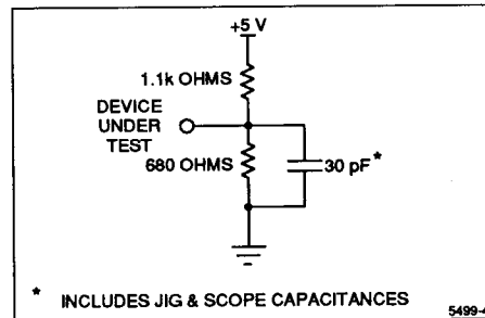
Figure 4. Output Load Caption
