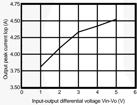
Figure 11. Output Peak Current vs. Input-Output Differential Voltage
