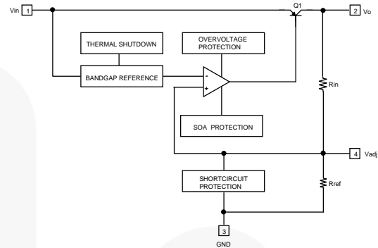
Figure 2. KA278RA05C
