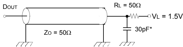
Output Loads(A)
