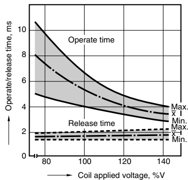
2. Operate/release time
