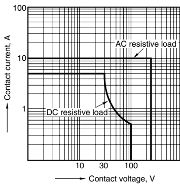
1. Maximum value for switching capacity
