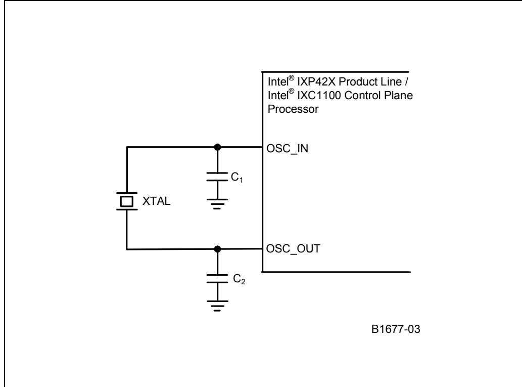
Figure 15. Typical Connection to an Oscillator
