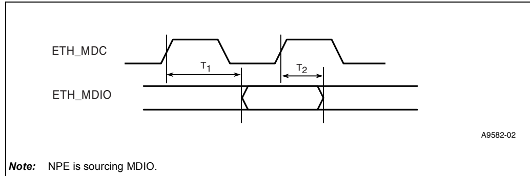
Figure 23. MDIO Input Timings
