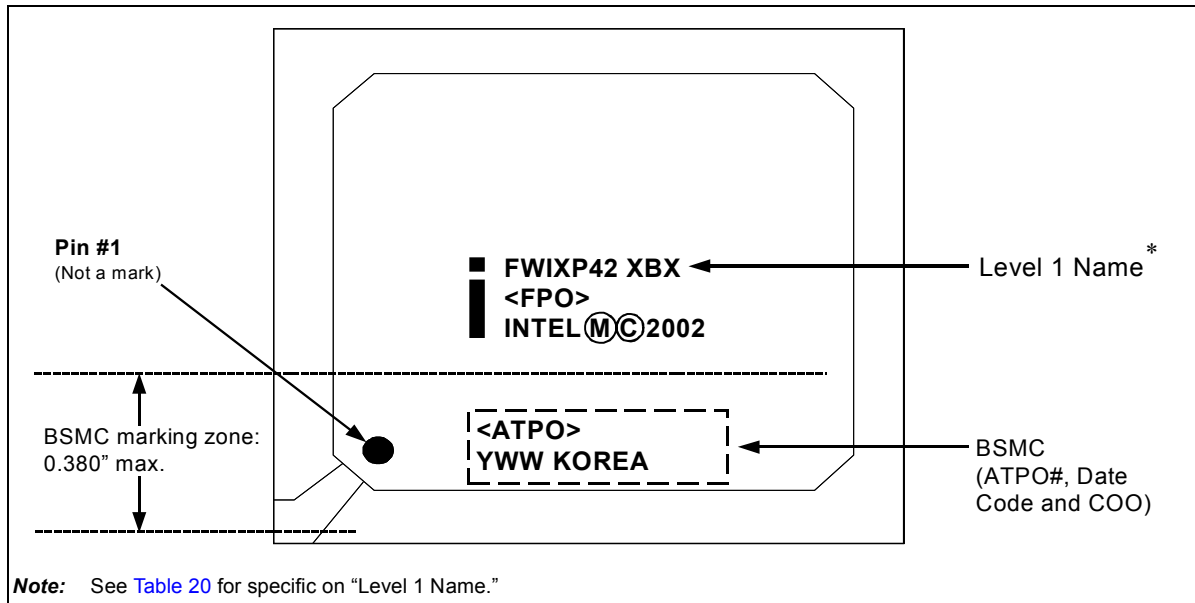
Figure 8. Package Markings
