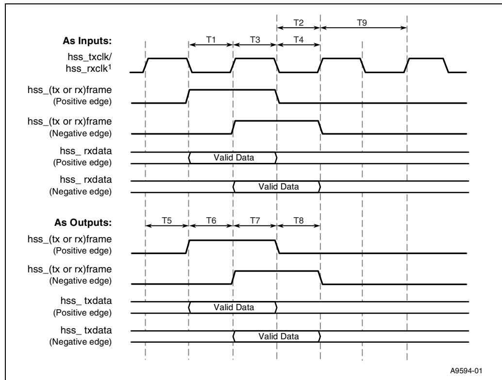
Figure 41. High-Speed, Serial Timings
