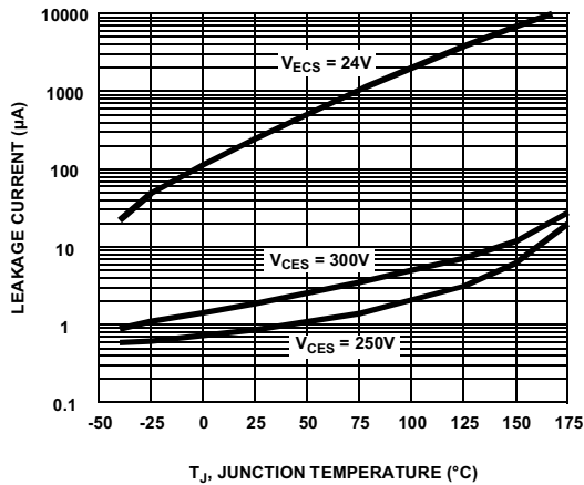
Figure 11. Leakage Current vs Junction Temperature
