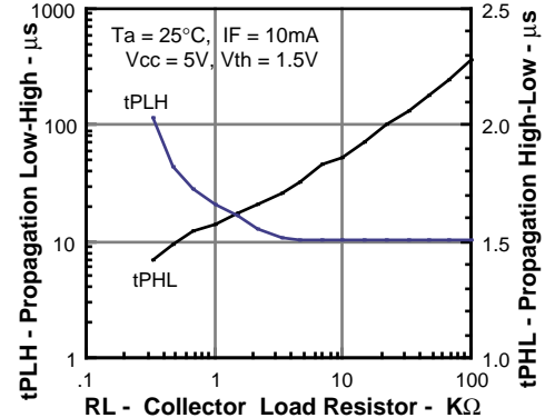
Figure 12. Propagation delay versus collector load resistor
