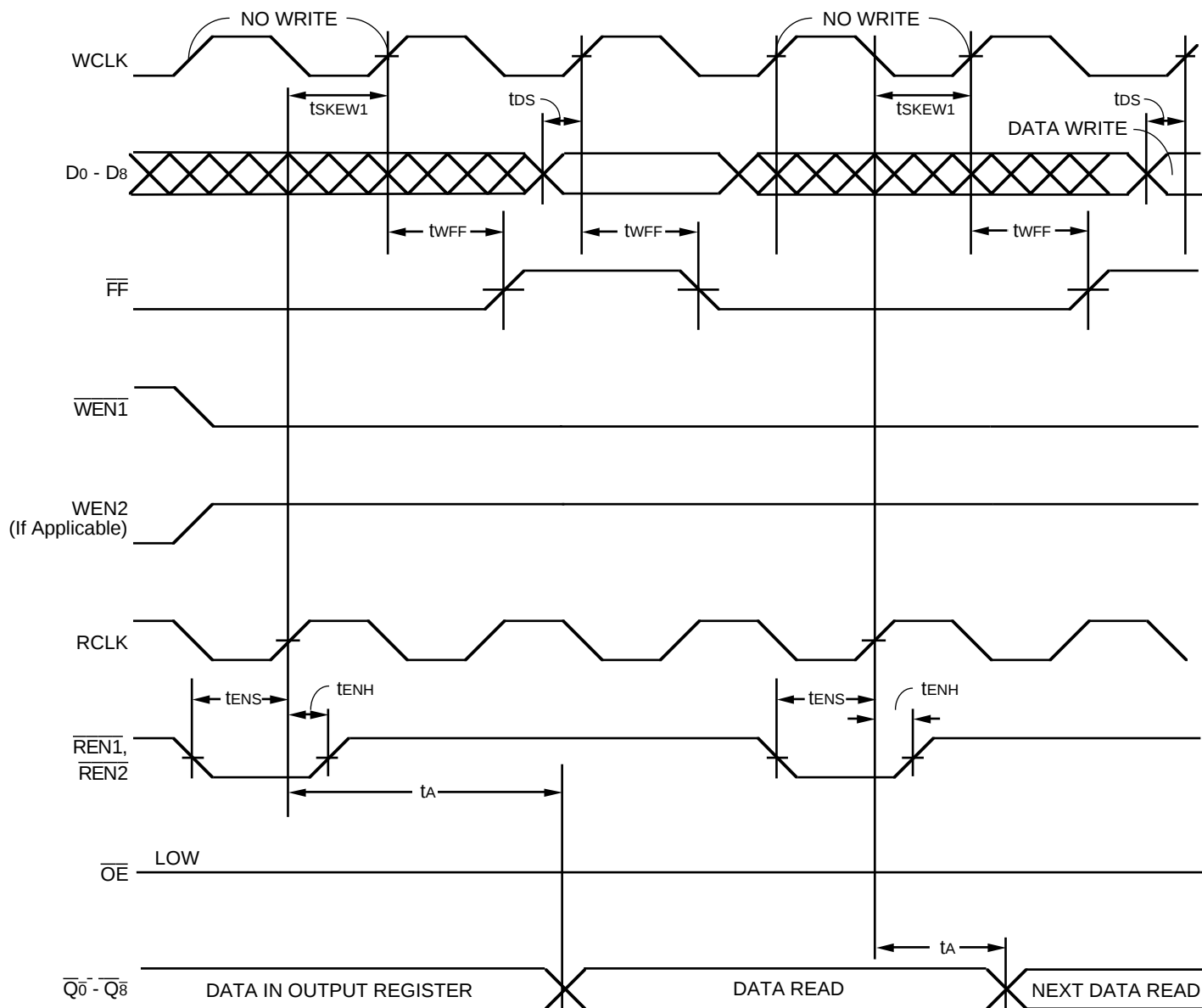
Figure 8. Full Flag Timing
