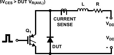
Figure 15. Avalanche Energy Test Circuit
