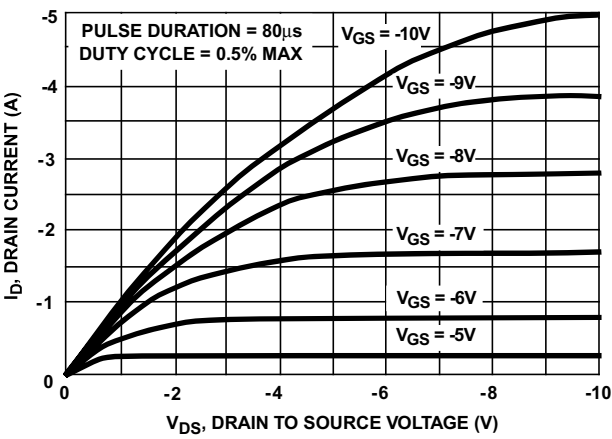
FIGURE 6. SATURATION CHARACTERISTICS
