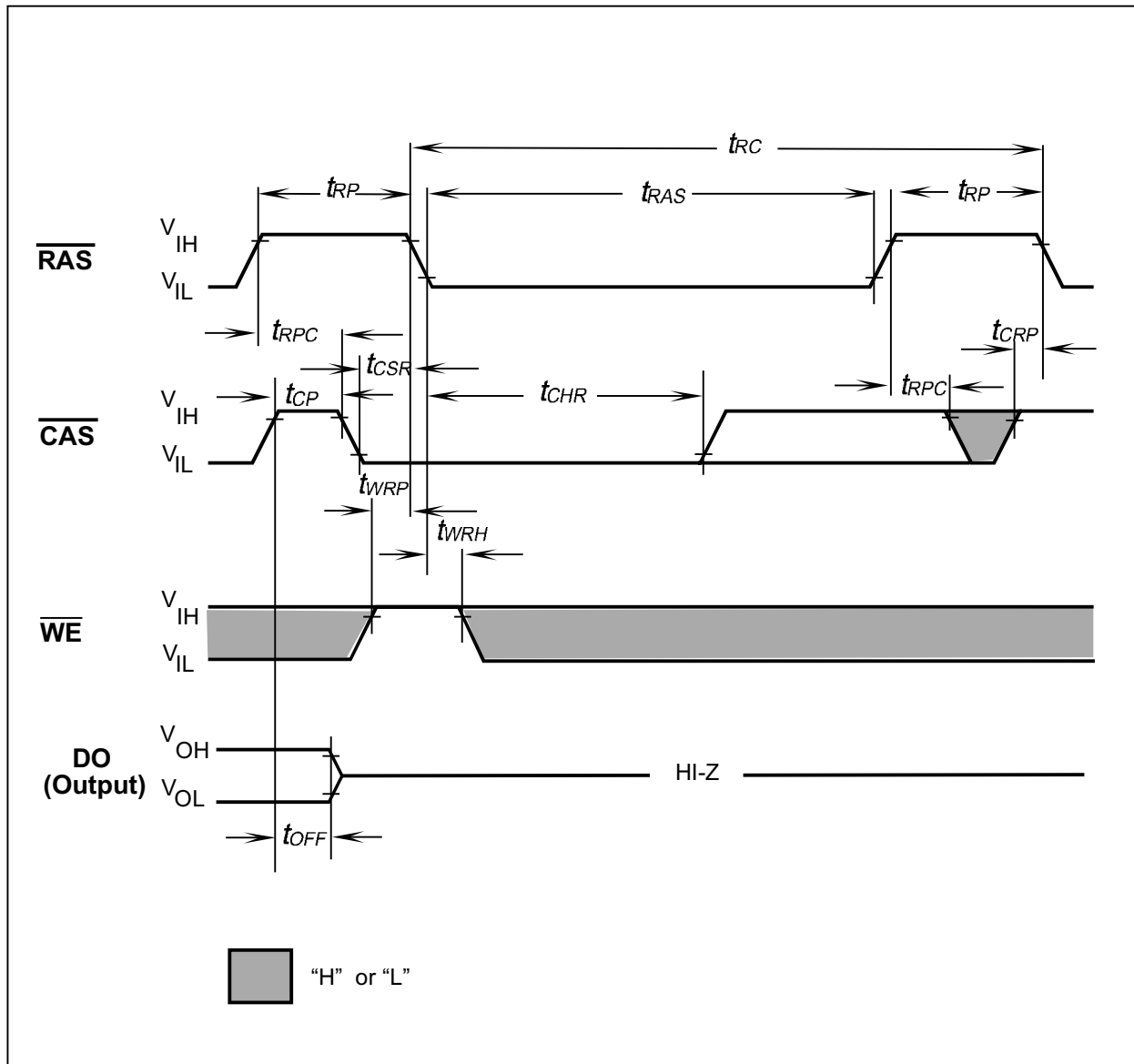
\overline{\text{CAS}} -Before- \overline{\text{RAS}} Refresh Cycle
