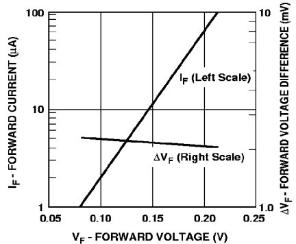
Figure 9. Typical V_f Match, HSMS-2860 Series Pairs at Detector Bias Levels.
