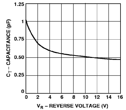
Figure 15. Total Capacitance vs. Reverse Voltage—HSMS-2810 Series.
