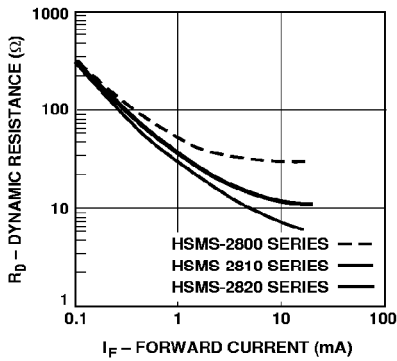
Figure 13. Dynamic Resistance vs. Forward Current—HSMS-2800 Series.
