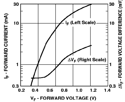
Figure 6. Typical V_f Match, HSMS-2820 Series Pairs and Quads at Mixer Bias Levels.
