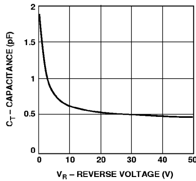
Figure 14. Total Capacitance vs. Reverse Voltage—HSMS-2800 Series.
