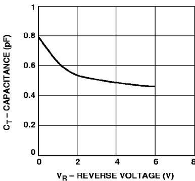
Figure 16. Total Capacitance vs. Reverse Voltage—HSMS-2820 Series.
