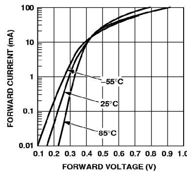
Figure 8. Typical Forward Current vs. Forward Voltage at Temperature, HSMS-2860 Series.
