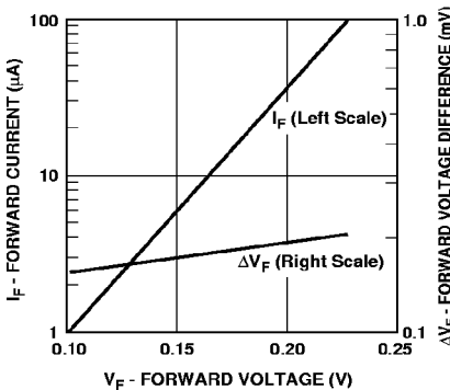
Figure 7. Typical V_f Match, HSMS 2820 Series Pairs at Detector Bias Levels.
