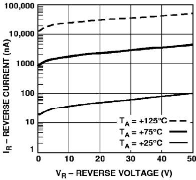
Figure 10. Reverse Current vs. Reverse Voltage at Temperatures—HSMS-2800 Series.
