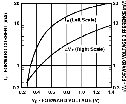
Figure 2. Typical V_f Match, HSMS-2800 Series Pairs and Quads.
