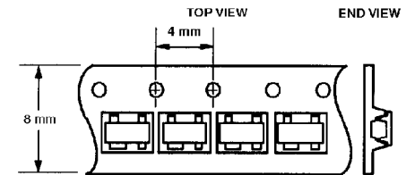
Figure 18. Option L31 for SOT-143 Packages.
