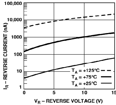
Figure 11. Reverse Current vs. Reverse Voltage at Temperatures—HSMS-2810 Series.
