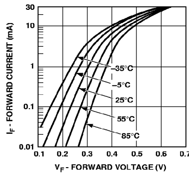
Figure 5. Typical Forward Current vs. Forward Voltage At Temperatures—HSMS-2820 Series.
