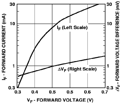
Figure 4. Typical V_f Match, HSMS-2810 Series Pairs and Quads.
