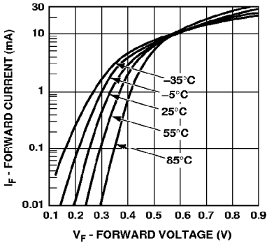
Figure 1. Typical Forward Current vs. Forward Voltage at Temperatures—HSMS-2800 Series
