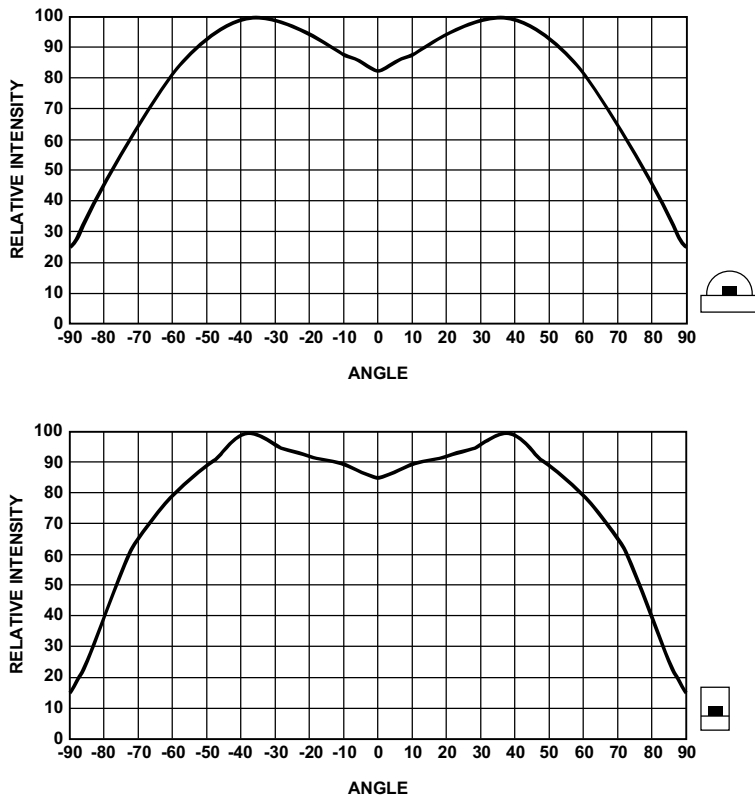
Figure 6. Relative Intensity vs. Angle for HSMx-C120.
