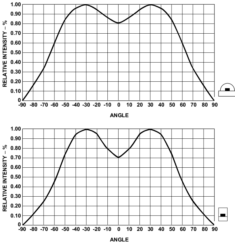
Figure 5. Relative Intensity vs. Angle for HSMx-C110.
