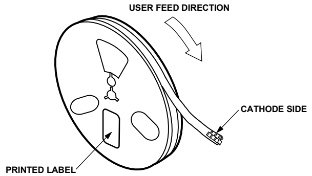
Figure 17. Reeling Orientation.
