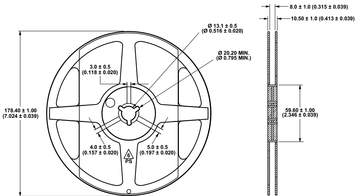
Figure 18. Reel Dimensions.
