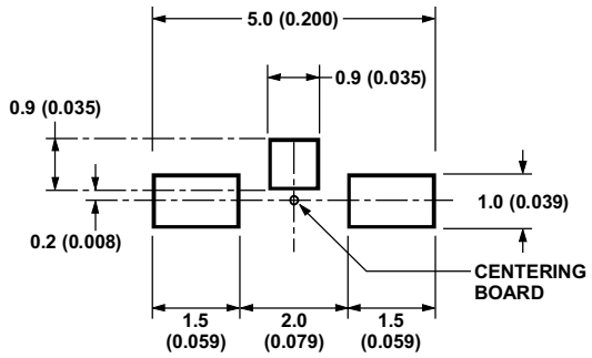
Figure 14. Recommended Soldering Pattern for HSMx-C110.
