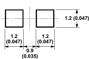
Figure 12. Recommended Soldering Pattern for HSMx-C170 and C177.
