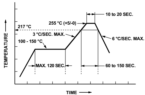
Figure 10. Recommended Pb-Free Reflow Soldering Profile.
