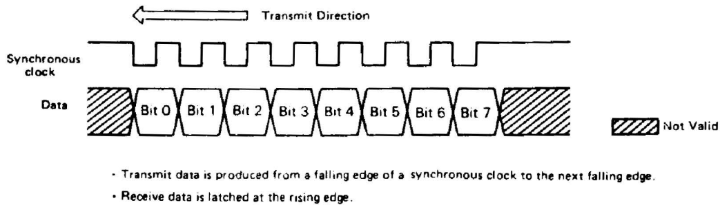
Figure 26 Clocked Synchronous Mode Format
