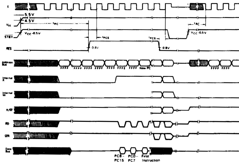
Figure 14 Reset Timing
