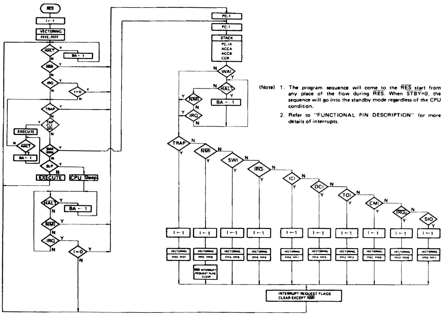
Figure 30 HD6303Y System Flow Chart
