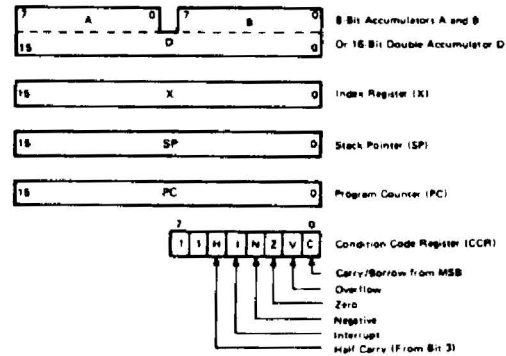
Figure 28 CPU Programming Model
