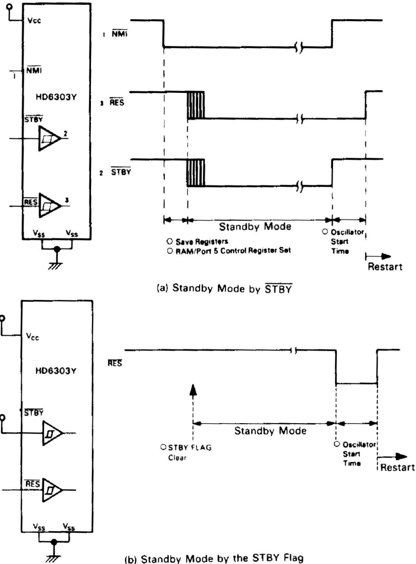
Figure 27 Standby Mode Timing
