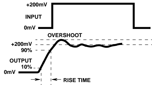
FIGURE 2. TRANSIENT RESPONSE
