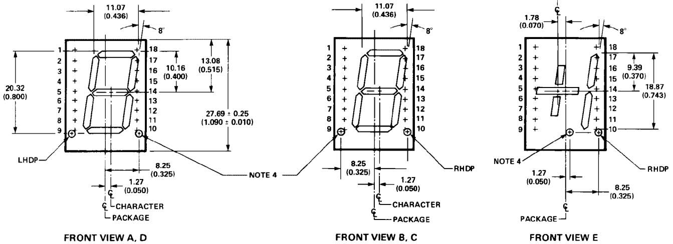
FRONT VIEW A, D
