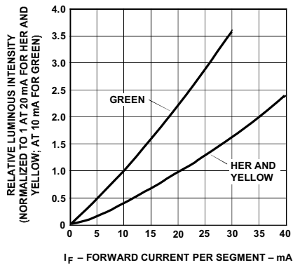
Figure 11. Relative Luminous Intensity vs. DC Forward Current.
