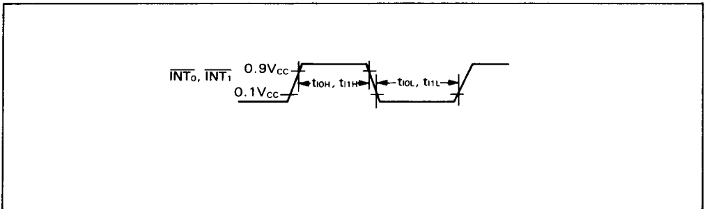
Figure 53. Interrupt Timing
