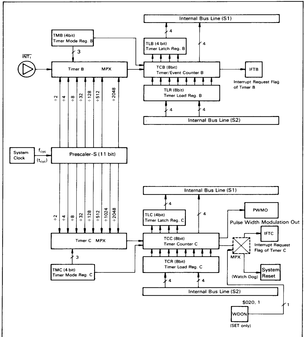
Figure 15. Timer B/Timer C Block Diagram
