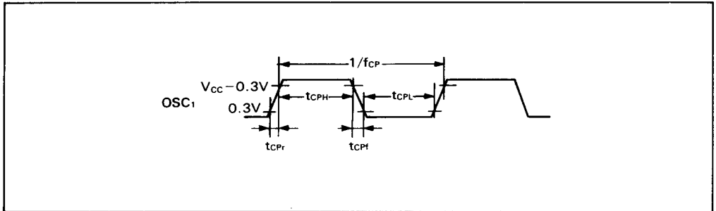
Figure 52. External Clock Timing
