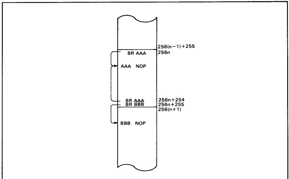
Figure 48. The Branch Destination by BR Instruction on the Boundary between Pages
