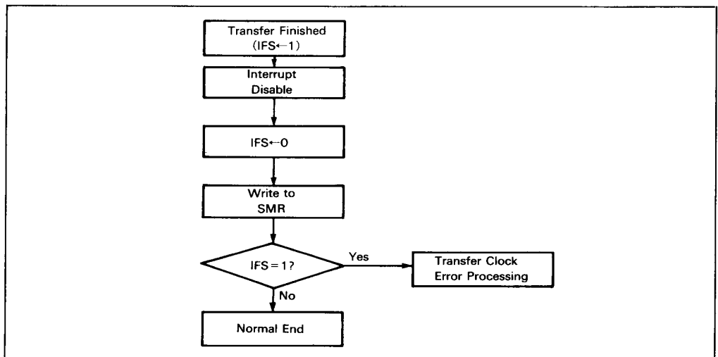
Figure 13. Example of Transfer Clock Error Detection
