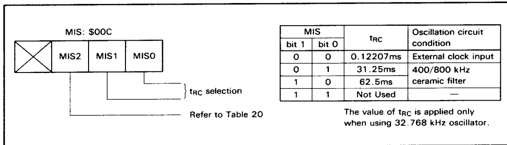
Figure 34. Miscellaneous Register
