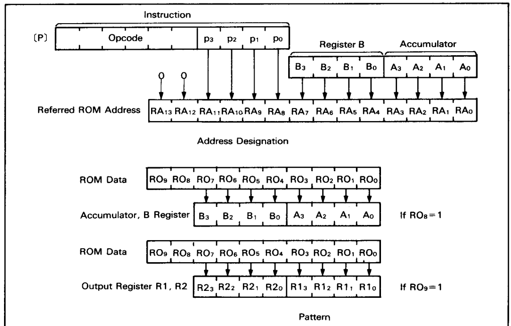
Figure 49. P Instruction
